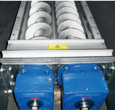
Double base frame screw model 360 for taking in material from the push floor systems etc. PUMPE's construction department specializes in custom solutions – just ask us!
