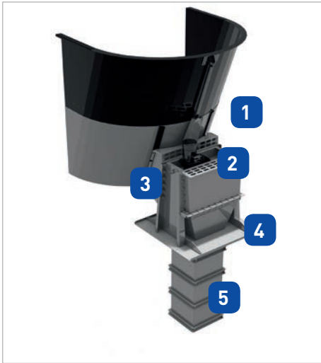
Fermenter screw model 600 vertical 1 Screw and drive according to ATEX 2 All stainless steel construction 3 Non-contract transfer from the biomixer to the fermenter screw 4 Mounting plate for fermenter cover 5 Stainless steel conveyor shaft
